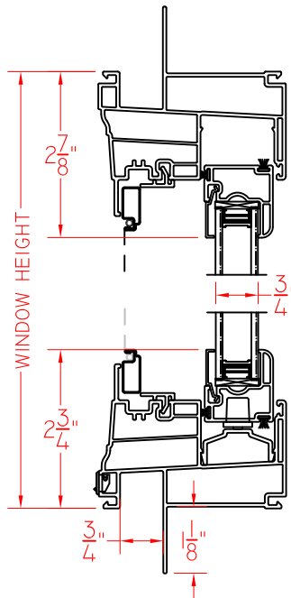
A VERTICAL CROSS SECTION
