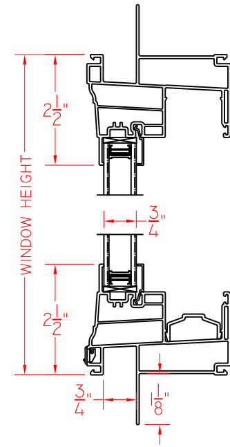
B VERTICAL CROSS SECTION
