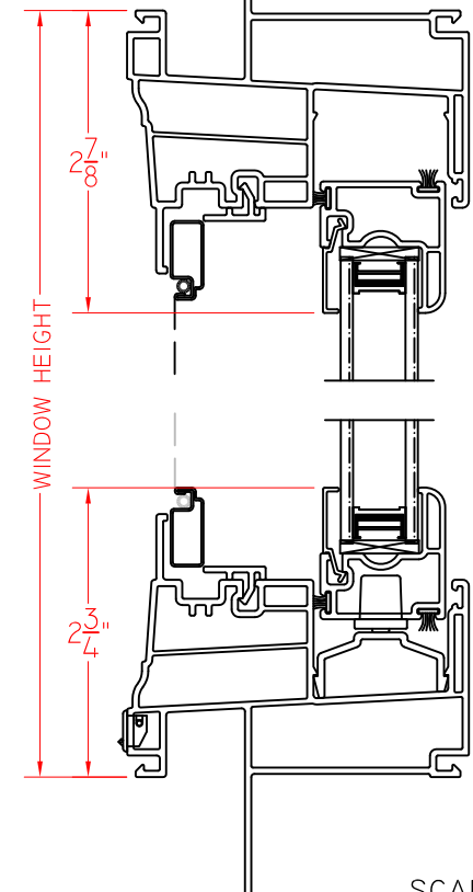
① B VERTICAL CROSS SECTION
