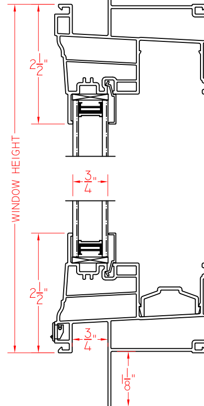
① A VERTICAL CROSS SECTION
